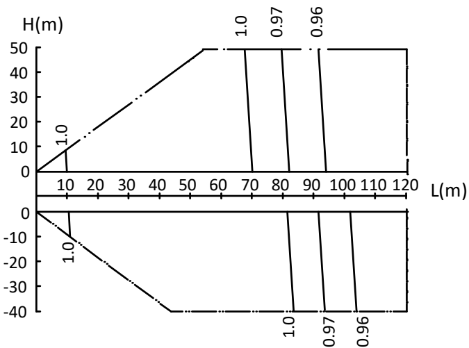
Rate of change in heating capacity
