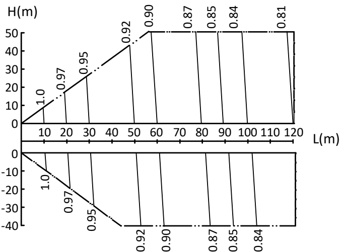
Rate of change in cooling capacity
