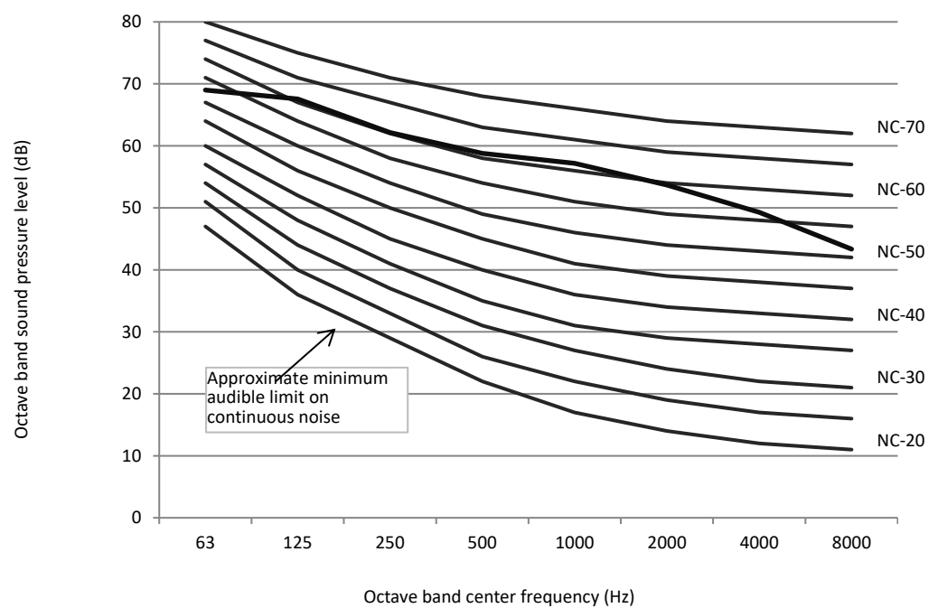
MDVOS-120HV2E octave band level
