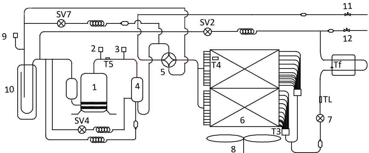
MDVOS-120HV2E piping diagram
