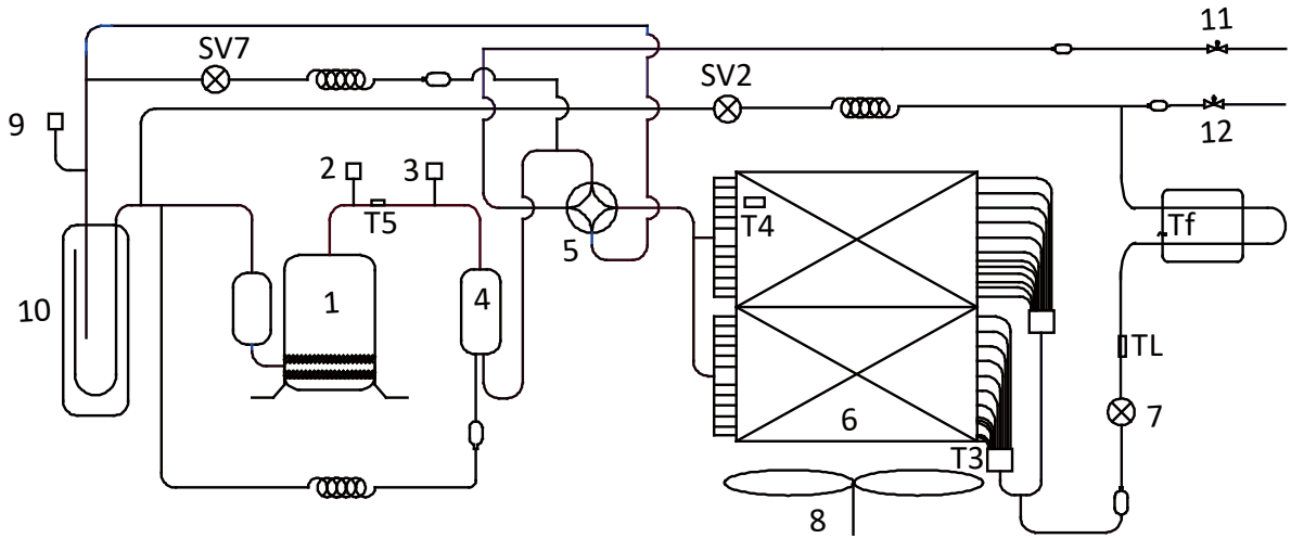
MDVOS-68HV2E; MDVOS-76HV2E; MDVOS-96HV2E piping diagram
